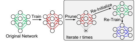
Figure 11: Leveraging lottery ticket hypothesis to prune DRL models. Lines with the same color indicate that the same parameters are used in neural networks.
