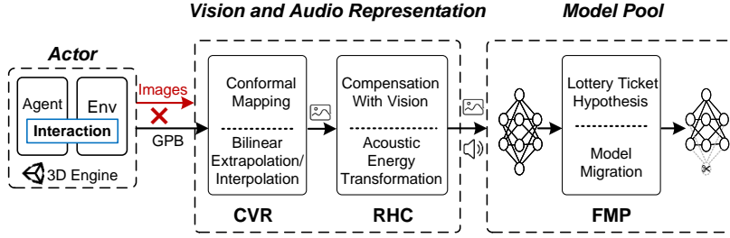
Figure 10: Architectural overview of ParliRobo.
